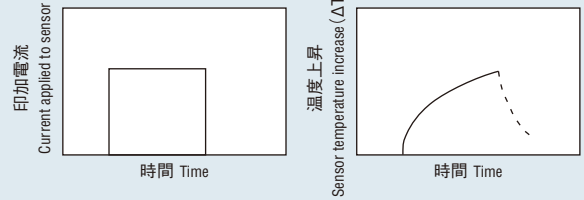
図3 昇温カーブと D(\tau) の関係 Fig. 3: Correlation between temperature increase curve and D(\tau)
